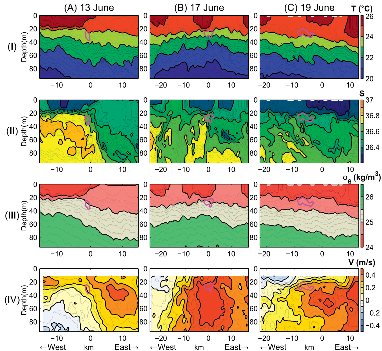
FIG. 9. Zonal sections of (top)–(bottom) temperature, salinity, potential density, and meridional velocity during the moderate-straining case study based on Triaxus and shipboard ADCP surveys at approximately (a) 1900 UTC 13 Jun, (b) 0500 UTC 17 Jun, and (c) 1240 UTC 19 Jun. The magenta contour shows the evolution of the rhodamine dye patch. The 13 Jun section location is marked with a dashed line in Fig. 8b; other sections were similarly positioned in the frame of reference advecting with the drifters. The distances are eastward relative to the center of mass of the drifter array.
