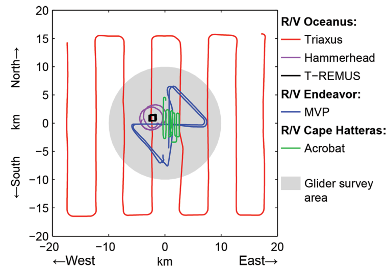
FIG. 3. Illustration of the nested sampling from R/V Oceanus (Triaxus, Hammerhead, and T-REMUS), R/V Endeavor (MVP), and R/V Cape Hatteras (Acrobat). Triaxus measured along a 30-km radiator grid (red), MVP made repeated 15-km bowtie surveys (blue), Acrobat performed adaptive surveying of the dye with a 3-km radiator grid, and Hammerhead was towed in 2-km-radius circles (magenta) around 1-km T-REMUS boxes (black) centered on a drogued Gateway buoy (not shown). Gliders surveyed within the 10-km-radius area on multiple intersecting tracks. Subsequent sampling patterns were shifted to keep up with the advection of dye and drifters.
