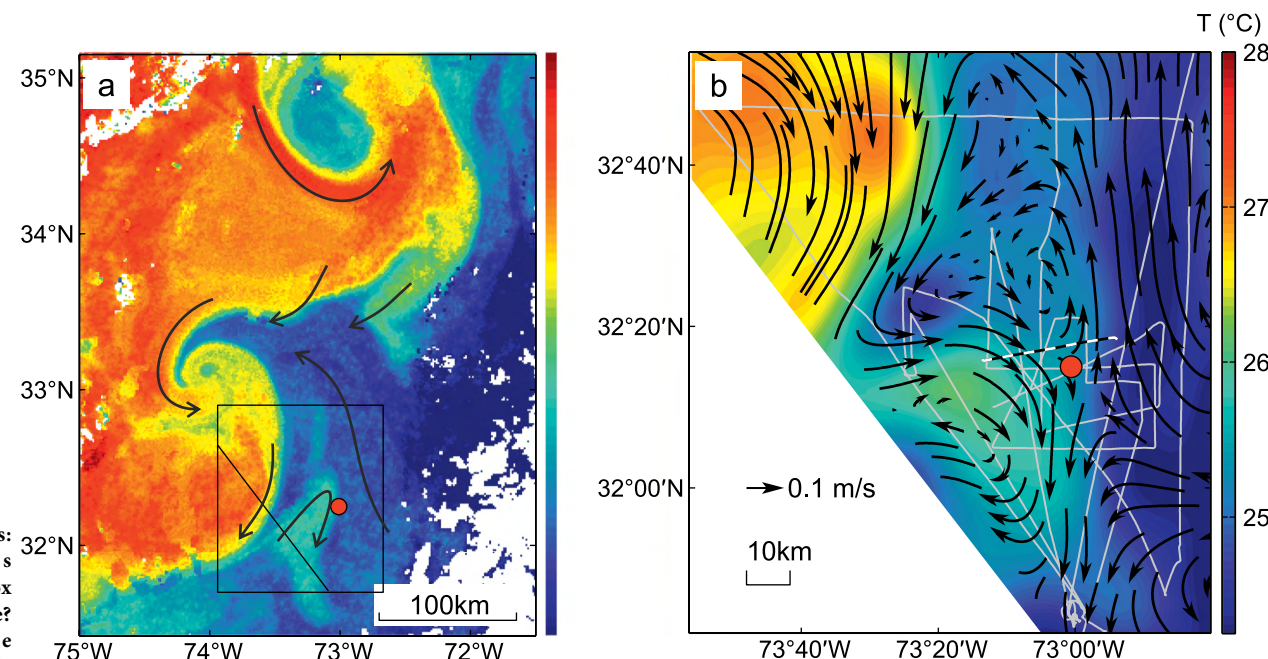
FIG. 8. Moderate-straining study area prior to the 13 Jun dye release. (a) AVHRR sea surface temperature image; black arrows show a subjective interpretation of the surface flow pattern. (b) Sea surface temperature and velocity field based on the reconnaissance survey carried out by all three vessels on 10–12 Jun 2011 (ship tracks are shown as white lines); the map extent is shown in (a). Red dots mark the flow stagnation (hyperbolic) point targeted by the study (see also Fig. 11). Zonal transect along the dashed line is shown in Fig. 9a.
