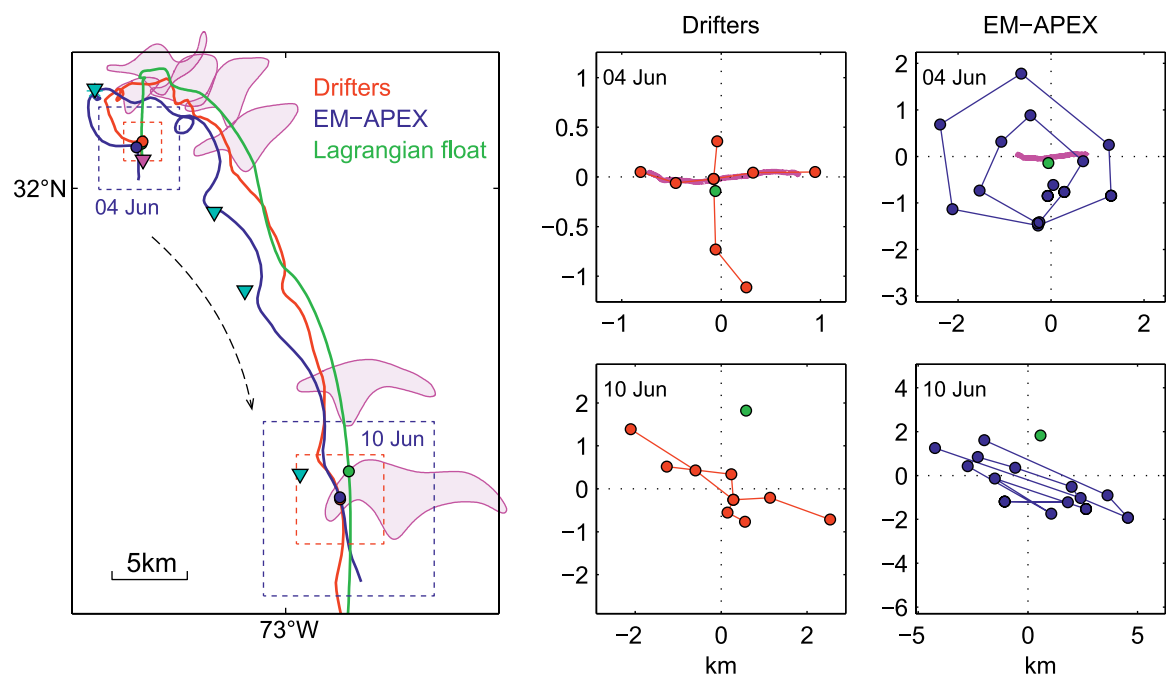
FIG. 6 (BOTTOM). Evolution and advection of the rhodamine dye patch and the arrays of drifters and floats during the weak-straining study on 4–10 Jun 2011. (left) The rhodamine patch (magenta), the trajectories of the centers of mass of the drifter array (red) and EM-APEX array (blue), and the interpolated trajectory of the Lagrangian float (green). The sites of rhodamine and fluorescein releases are marked with magenta and cyan triangles, respectively. (right) The configuration of the arrays at the beginning of the study (0700 UTC 4 Jun 2011) and at the end (0000 UTC 10 Jun 2011). The location and extent of each panel is marked on the left with the dashed lines (red for drifters and blue for EM-APEX). North and east distances are relative to the centers of mass of the drifter arrays. A few EM-APEX floats were omitted for clarity. The magenta lines in the 4 Jun panels show the initial rhodamine dye streak.
