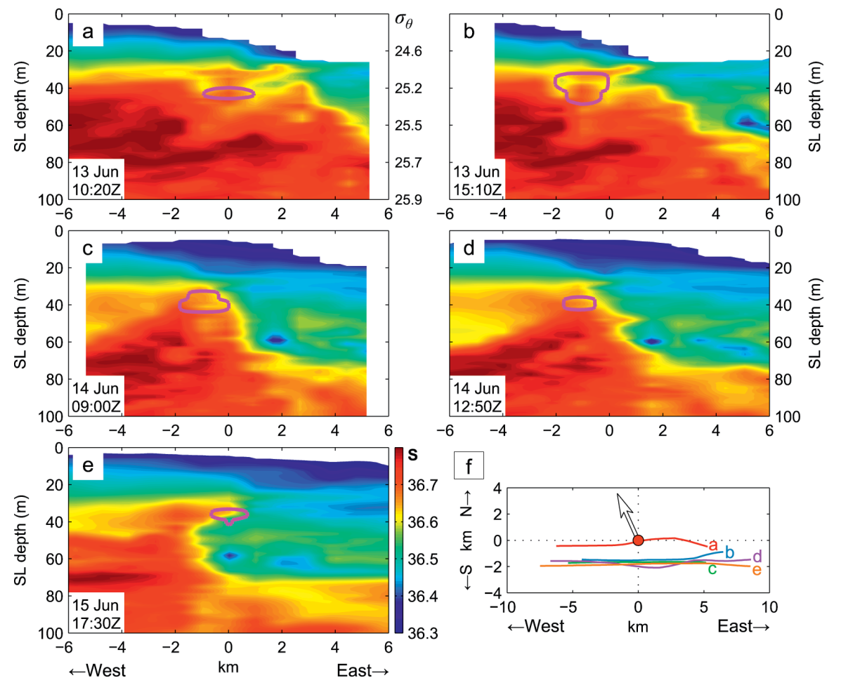
FIG. 10. (a)–(e) High-resolution zonal MVP sections showing evolution of a north–south-oriented thermohaline (spice) front in the vicinity of the rhodamine dye patch during 13–15 Jun 2011 under a \sim 0.1\text{-f} confluence. The vertical axis is an isopycnal (semi-Lagrangian) depth: namely, the average depth of an isopycnal, and corresponding potential density values are marked on the right in (a). The magenta contour shows evolution of the rhodamine dye patch. (f) Location of sections shown in (a)–(e) in the advected frame of reference moving with the center of mass of the drifter array (red circle). The arrow shows the mean advection direction during 13–15 Jun.
