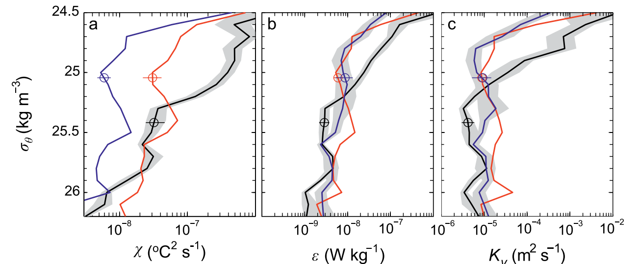
FIG. 15. Average diapycnal profiles of (a) thermal variance dissipation rate, (b) turbulent kinetic energy dissipation rate, and (c) diapycnal eddy diffusivity derived from the three deployments of microstructure EM-APEX floats in weak-straining (3–10 Jun: black) and moderate-straining (12–16 Jun: red; 16–19 Jun: blue) case studies. The shading shows 95% confidence intervals. The circles and horizontal bars are values and confidence intervals at the target isopycnals of rhodamine dye releases.
