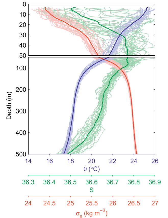
FIG. 1. Profiles of potential temperature (blue), salinity (green), and potential density (red) during LatMix Seaglider deployment 3–10 Jun 2011. Heavy lines indicate the mean profiles. Salinity is reported on the practical salinity scale throughout (nondimensional).
